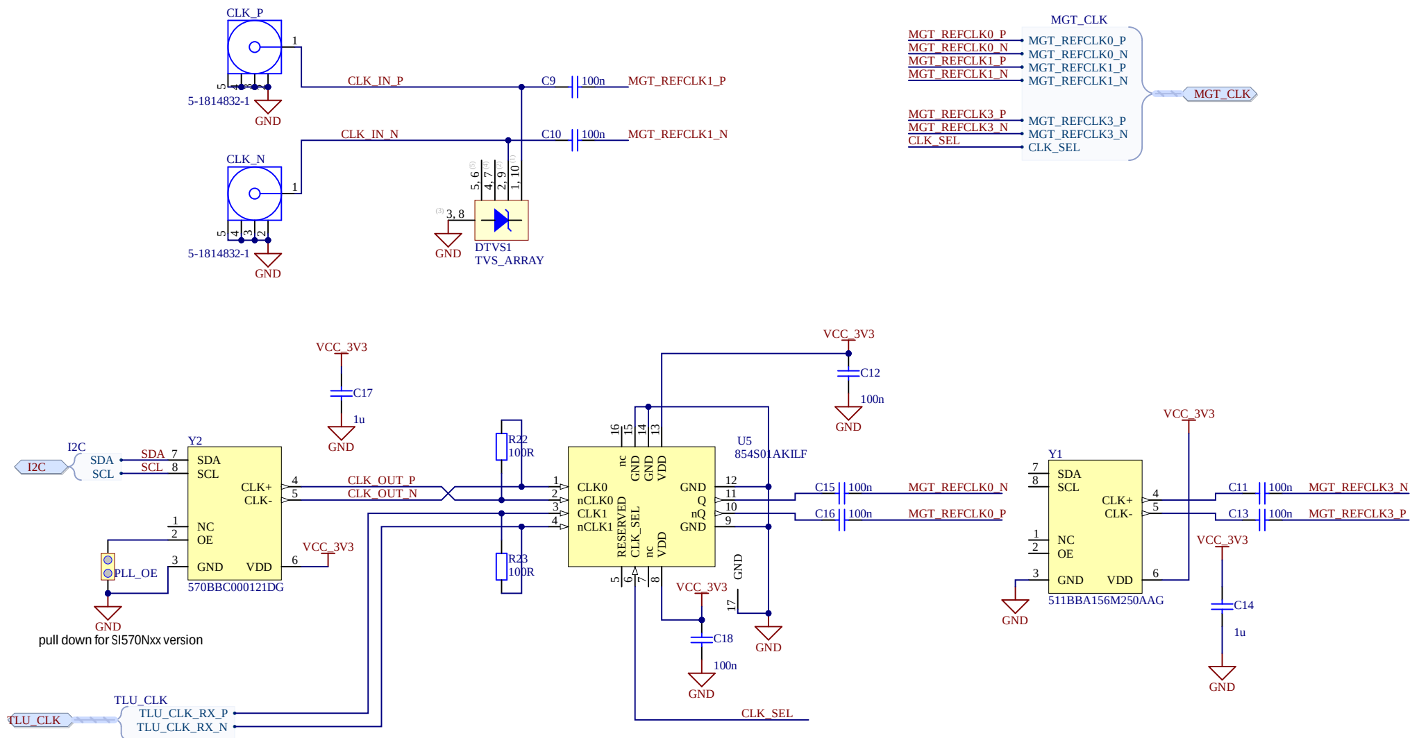
Ref Clk Oscillator, Multiplexer, SMA
